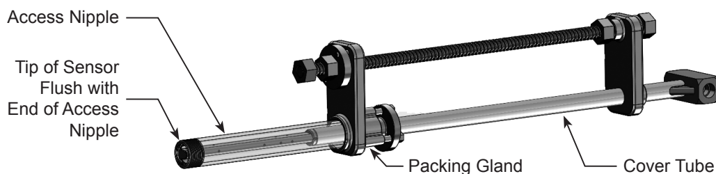
Figure 3. Access Nipple
